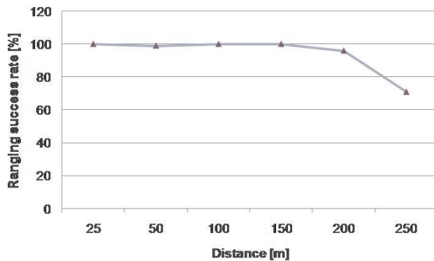
Figure 6 Range measurement between a pedestrian and a car
