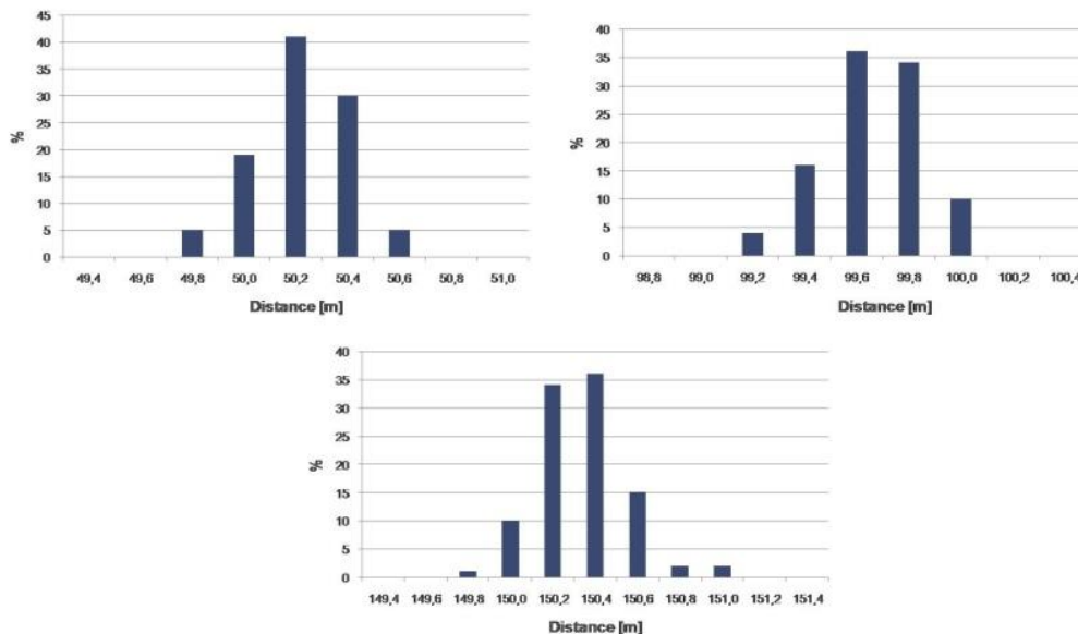
Figure 5 Ranging Accuracy - Ranging Accuracy is characterized by offset and spread. The actual distances are 50, 100, and 150m respectively
