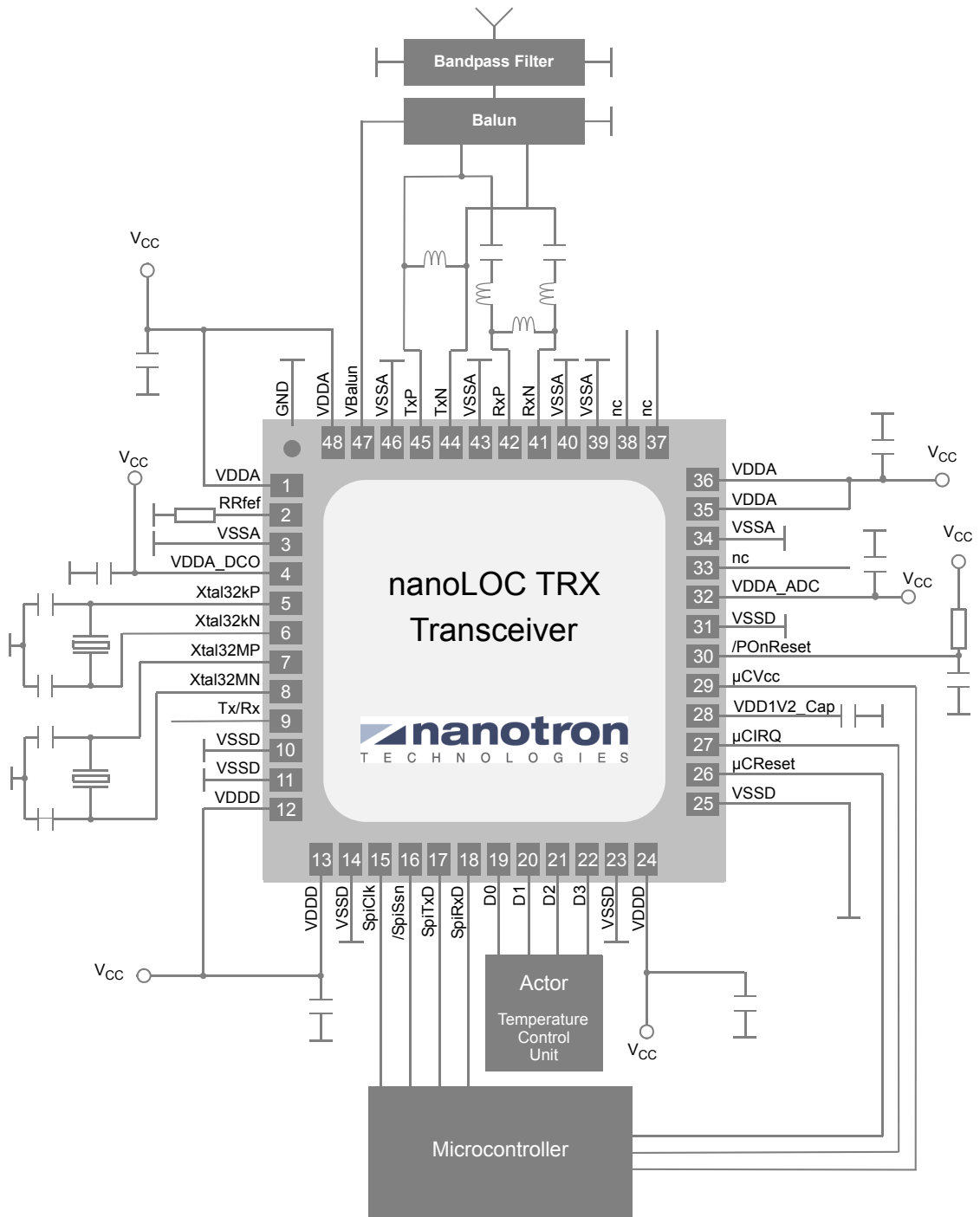
Sample application showing recommended circuitry
